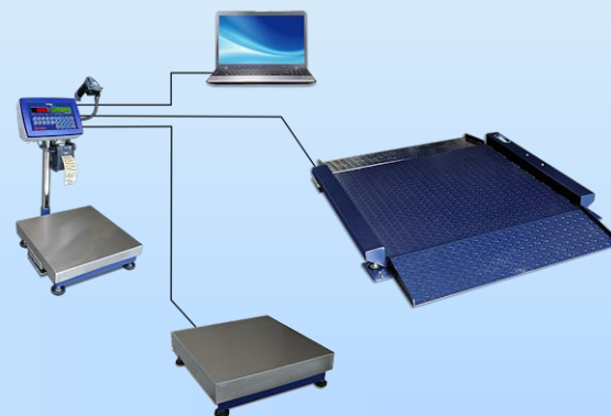
Schematic example of a network with various weighing platforms linked to the weighing indicator HP-Ultra, where the weighing data can be communicated to a laptop or PC.
